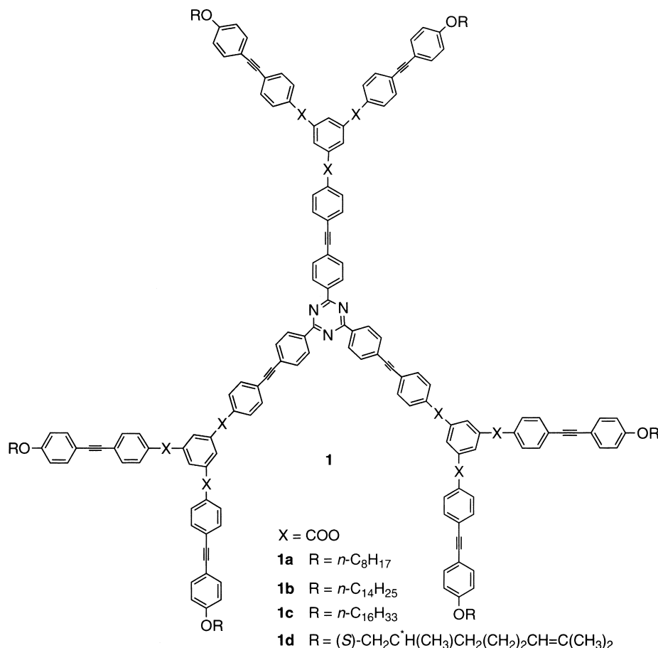
Scheme 1. Structure of star-shaped discotic liquid crystal.
