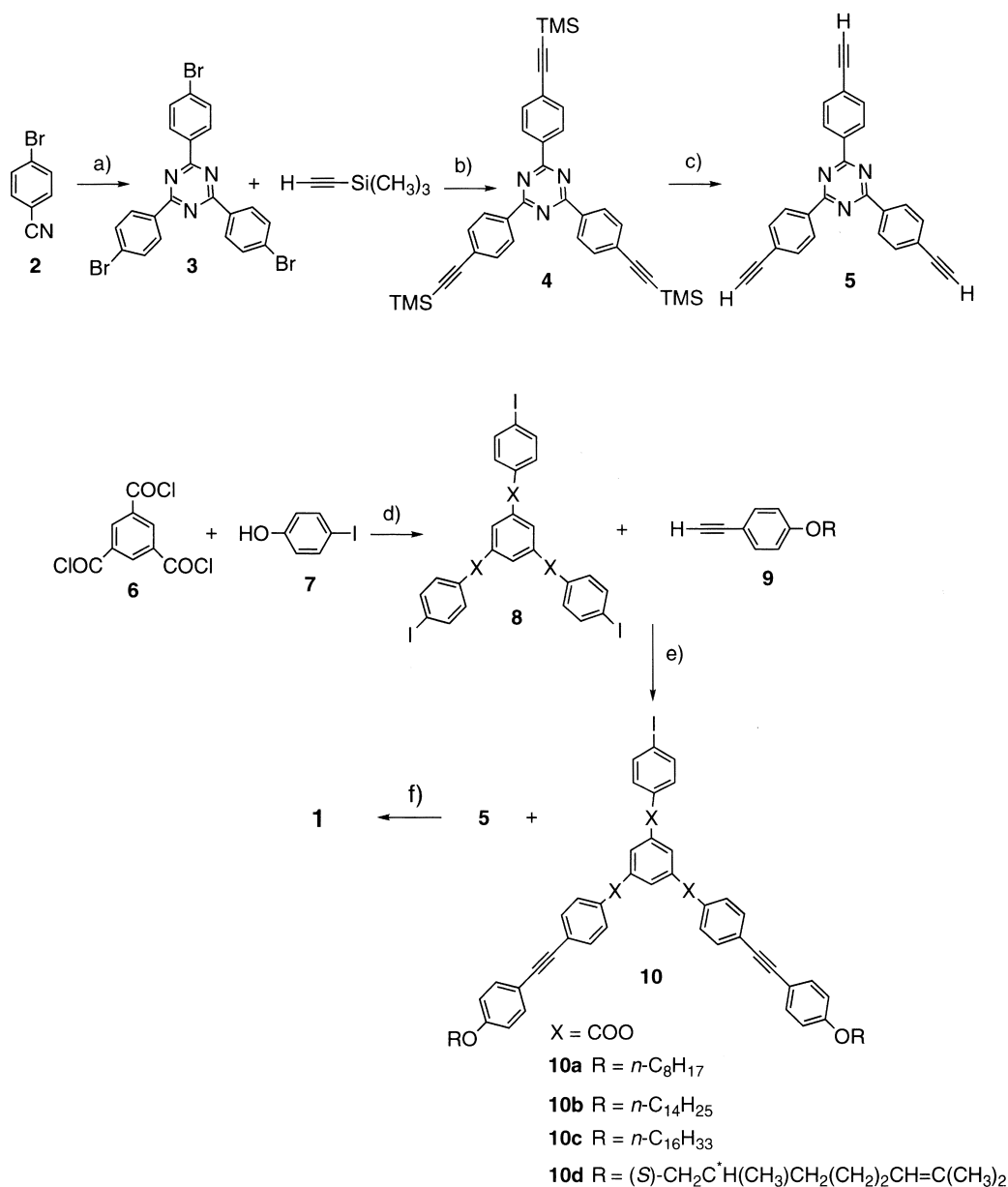
Scheme 2. a) \text{CF}_3\text{SO}_3\text{H} , \text{CHCl}_3 , r. t. b) \text{NEt}_3 , \text{CuI} , [\text{Pd}(\text{PPh}_3)_4] , THF, 55 °C. c) tetrabutylammonium fluoride, THF, r.t. d) \text{NEt}_3 , THF, r.t. e) \text{NEt}_3 , \text{CuI} , [\text{Pd}(\text{PPh}_3)_4] , THF, 55 °C. f) \text{NEt}_3 , \text{CuI} , [\text{Pd}(\text{PPh}_3)_4] , toluene, 60 °C.
